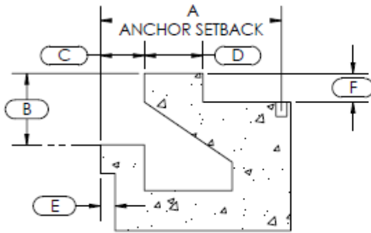
RECESSED GUTTER*
