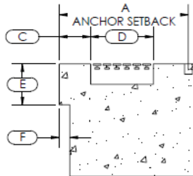
RIM FLOW GUTTER*
