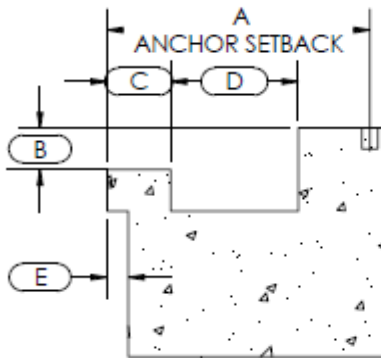
TROUGH GUTTER*
