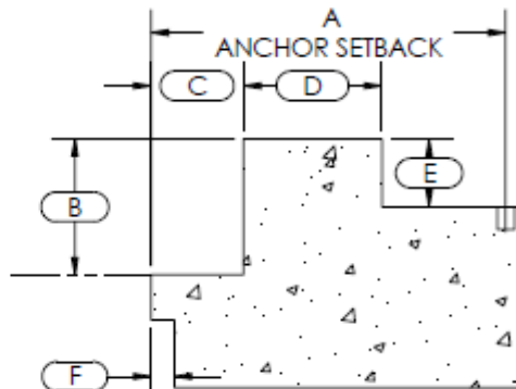
HAUNCH GUTTER*
